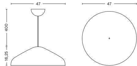
PAO STEEL PENDANT 470 DIAMETER 47 CM | 18.5" HEIGHT 16,25 CM | 6.4"
