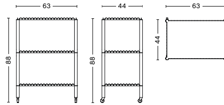
ARCS TROLLEY HIGH WIDTH 44 CM LENGTH 63 CM HEIGHT 88 CM
