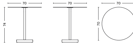
TERRAZZO TABLE ROUND DIAMETER Ø70 CM HEIGHT 74 CM
