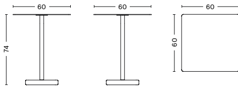
TERRAZZO TABLE SQUARE LENGTH 60 CM WIDTH 60 CM HEIGHT 74 CM
