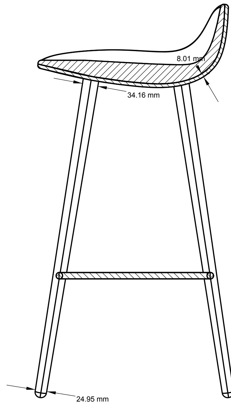
Section C-C
