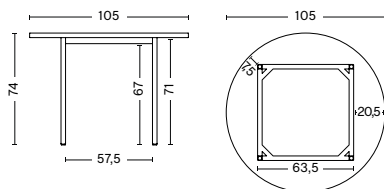
DIAMETER 105 CM HEIGHT 74 CM
