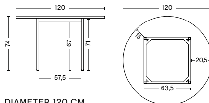
DIAMETER 120 CM HEIGHT 74 CM
