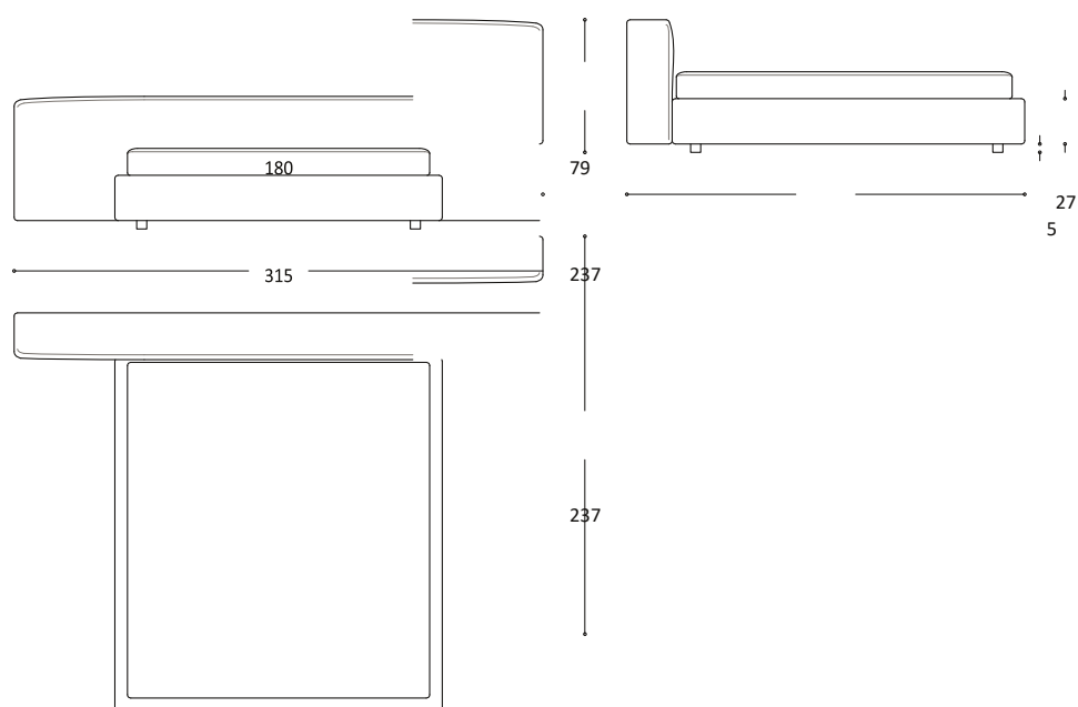
Bed for slat cm 180x200
