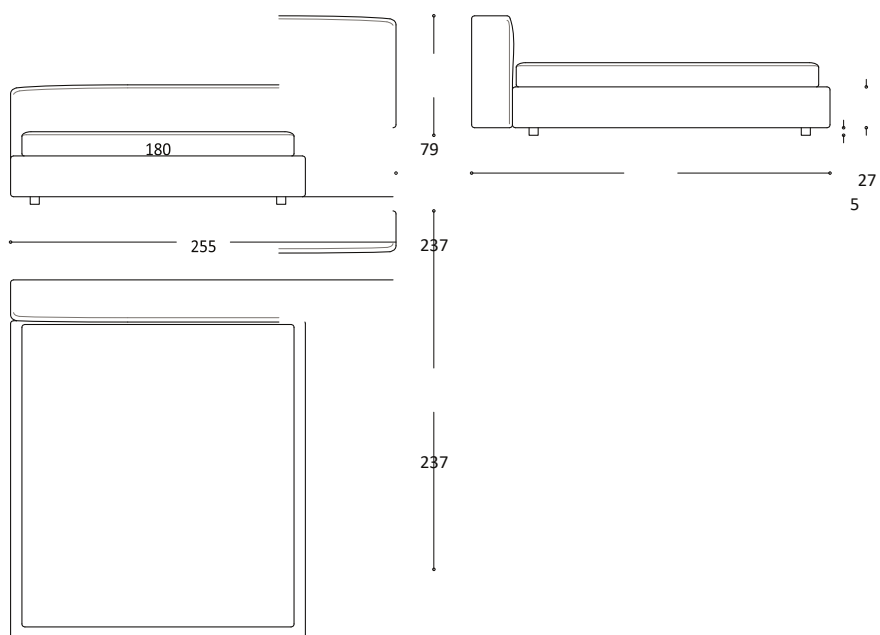
Bed for slat cm 180x200
