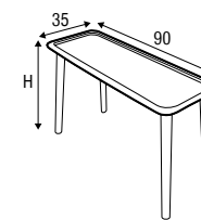
side table 90x35 h-55/38/45
