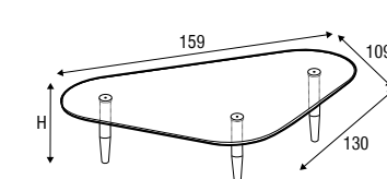
coffee table 130x130 h-40/45/55
