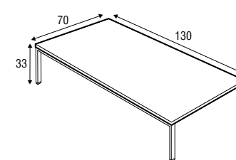
coffee table 130x70 h-33
